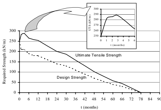
Figure 6. Ultimate Limit State analyses for safety factors = 1.0.
